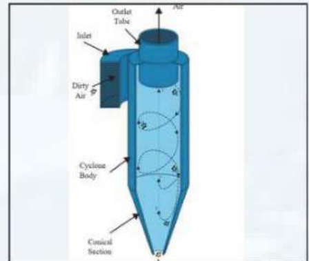
CYCLONE SEPERATOR
